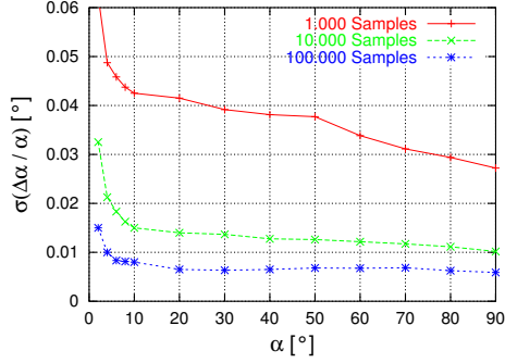
Fig. 6. Mixture of two Laplacian source signals with identical variances for different number of samples. The standard deviation of \Delta\alpha/\alpha calculated from 100 runs for each angle \alpha is plotted.
