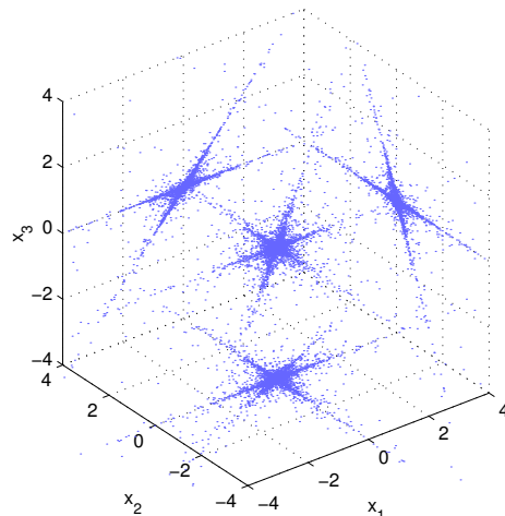
Fig. 8. Projection of a three dimensional mixture of Laplacian signals onto the three coordinate planes. Note that the projection into the x_1 - x_2 -plane does not have two distinct lines which are needed for the geometric algorithms.
